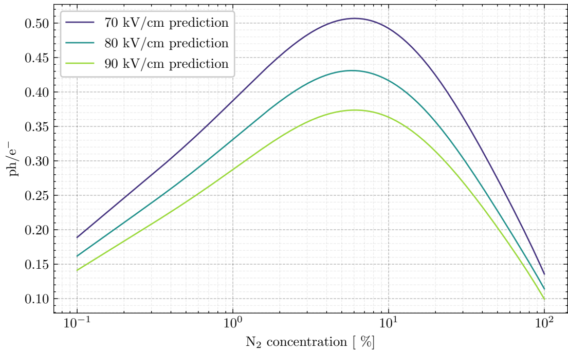
1 bar 10k gain secondary yield prediction for Ar/N 2 mixture
