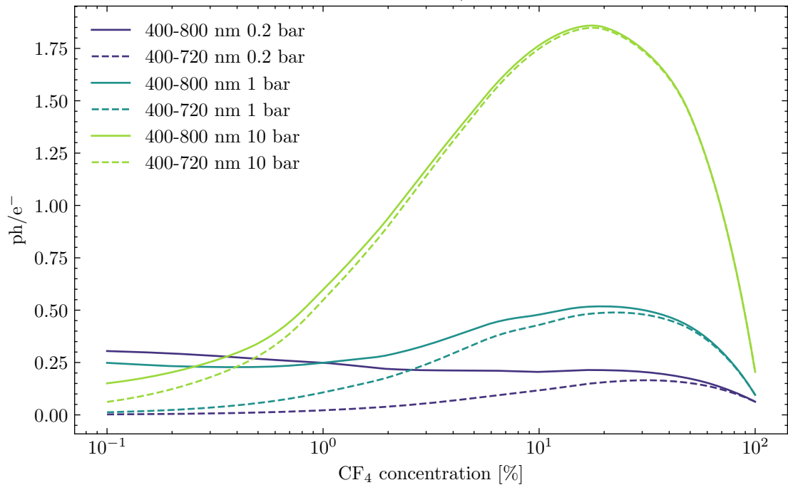
Secondary Yield Prediction for Ar/CF mixture GEM 100 gain
