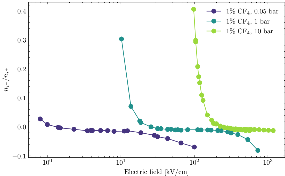
Estimated n_{i-}/n_{i+} for Ar/CF 4 , 1% CF 4
