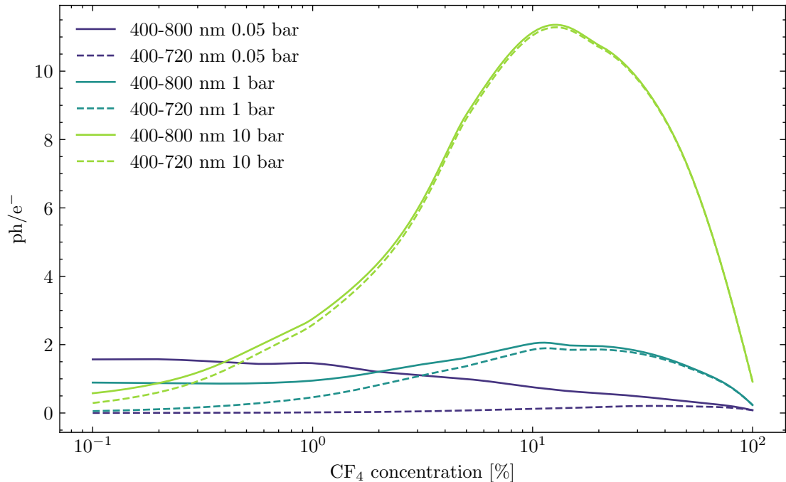
Secondary Yield Prediction for Ar/CF mixture thGEM 100 gain
