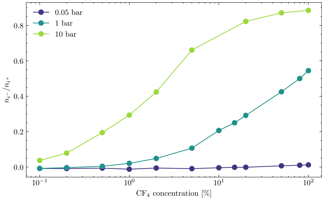
Estimated n_{i-}/n_{i+} for Ar/CF 4 thGEM
