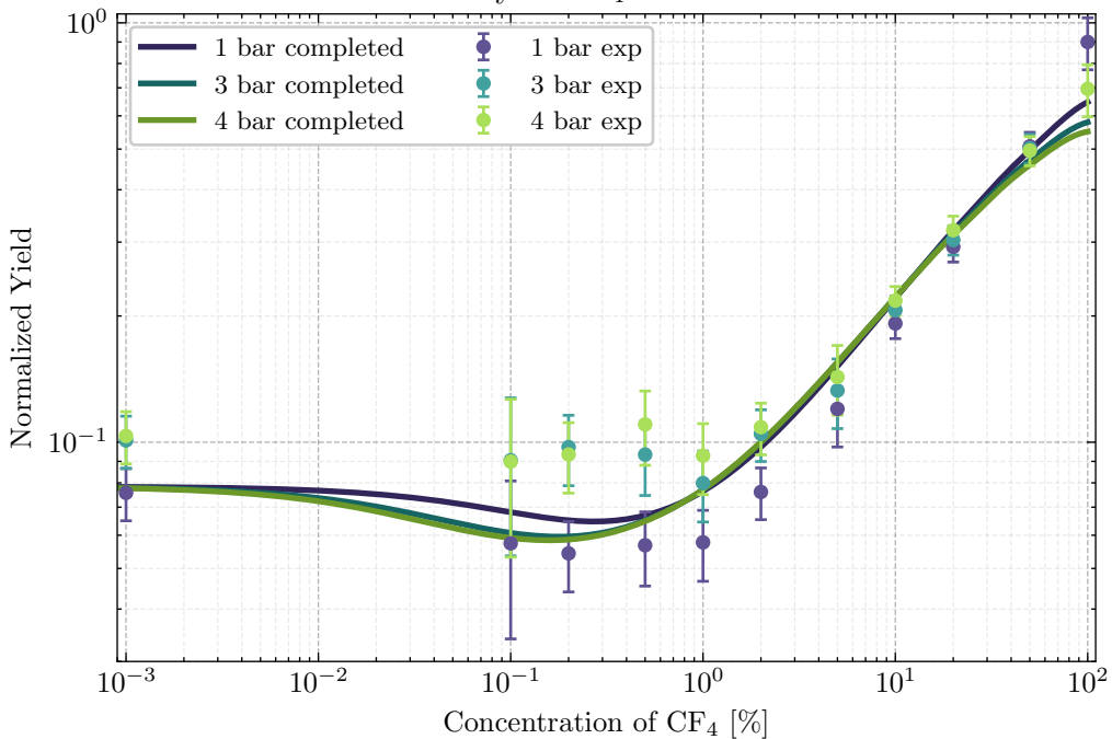
Primary ArCF 4 UV Yield fit
