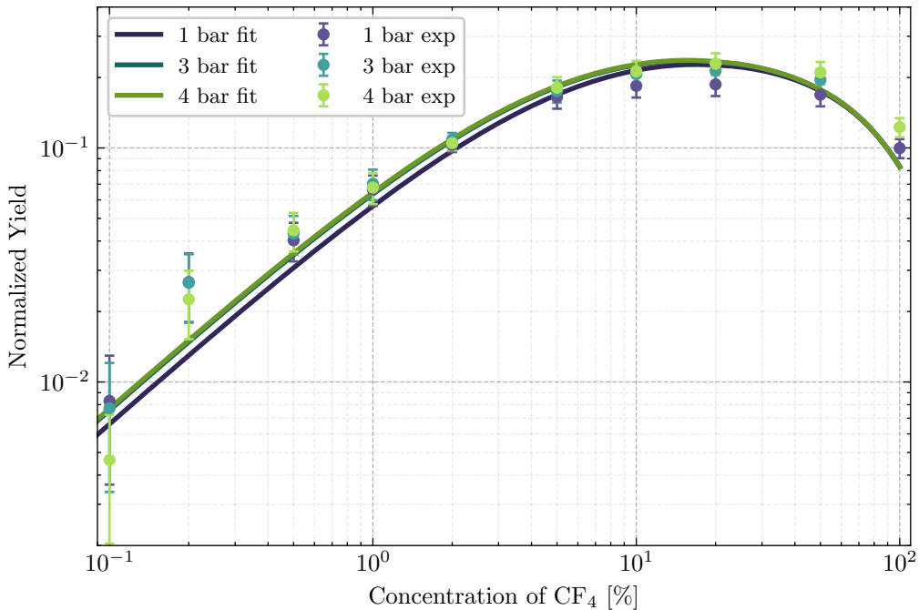
Primary ArCF 4 Visible Yield fit
