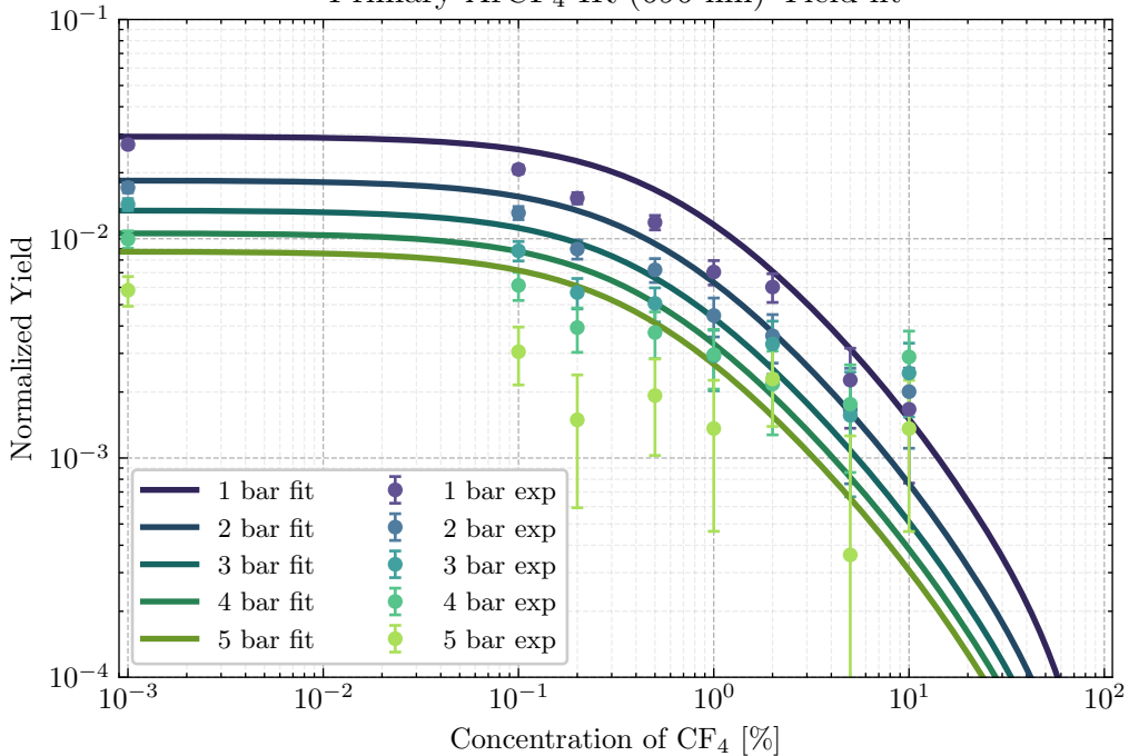
Primary ArCF 4 IR (696 nm) Yield fit
