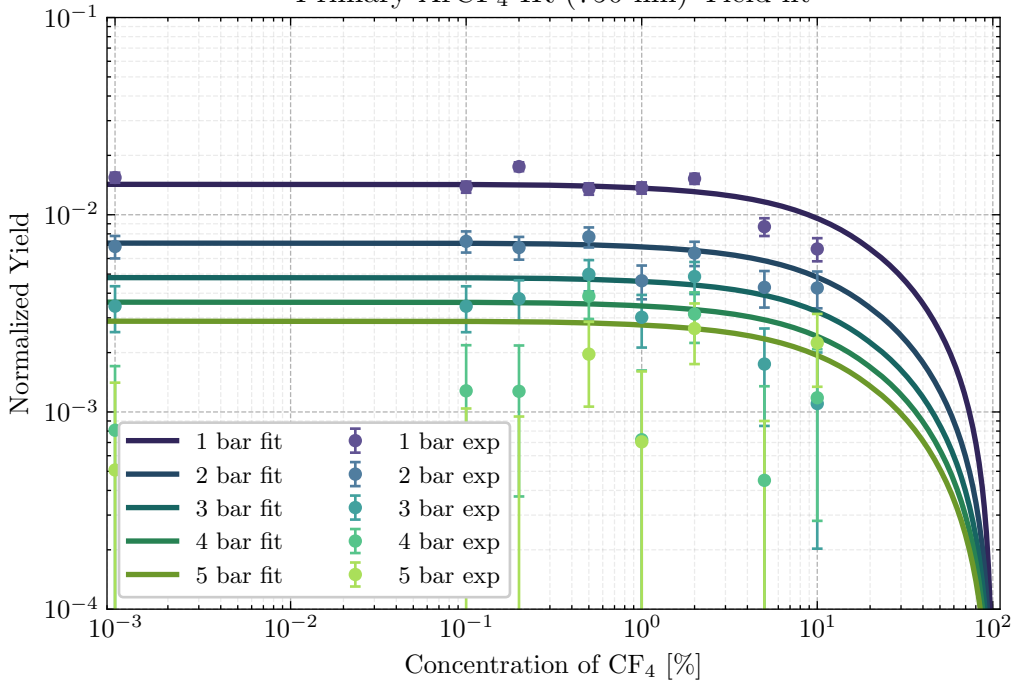
Primary ArCF 4 IR (750 nm) Yield fit
