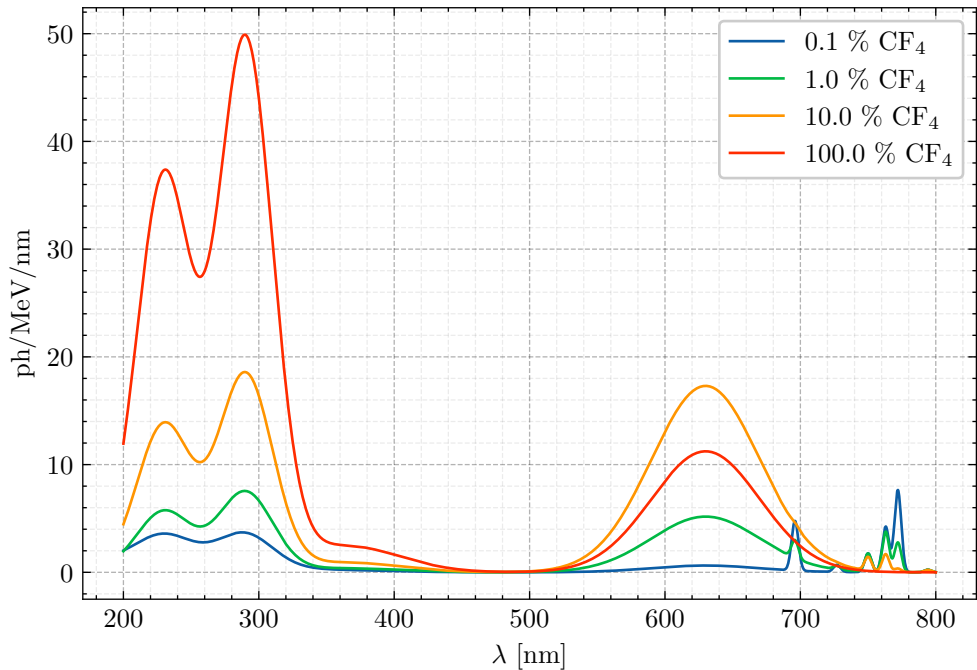
Primary Ar-CF 4 Spectra Prediction 10.0 bar
