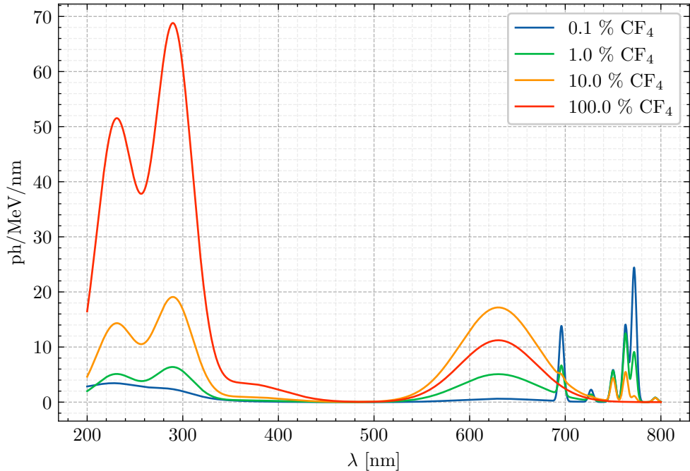
Primary Ar-CF 4 Spectra Prediction 3.0 bar
