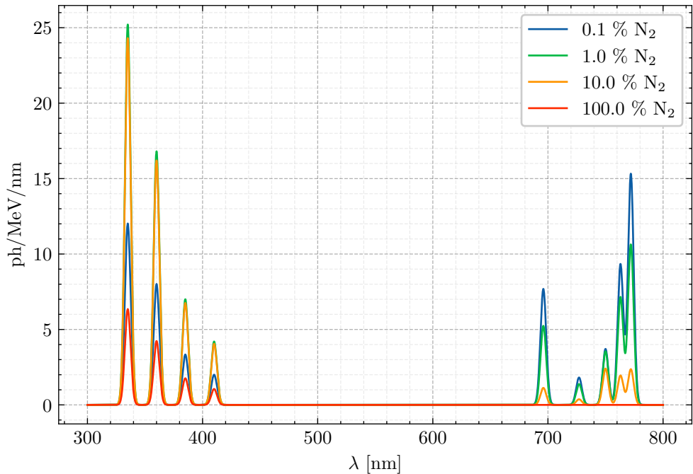
Primary Ar-N 2 Spectra Prediction 2.0 bar
