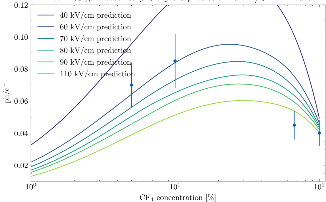
1 bar 100 gain secondary UV yield prediction for Ar/CF 4 mixture
