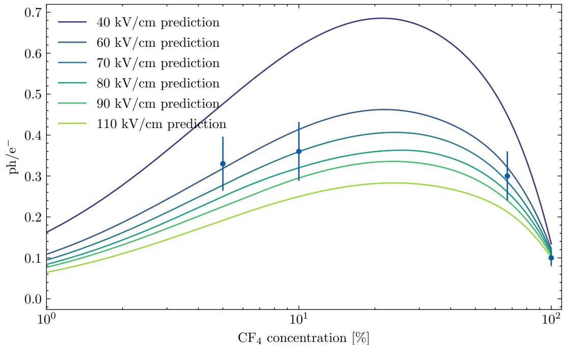
1 bar 100 gain secondary visible yield prediction for Ar/CF4 mixture
