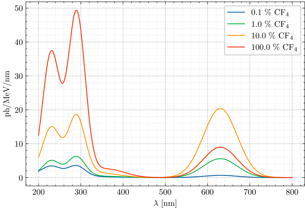
Primary Ar-CF 4 Spectra Prediction 10.0 bar
