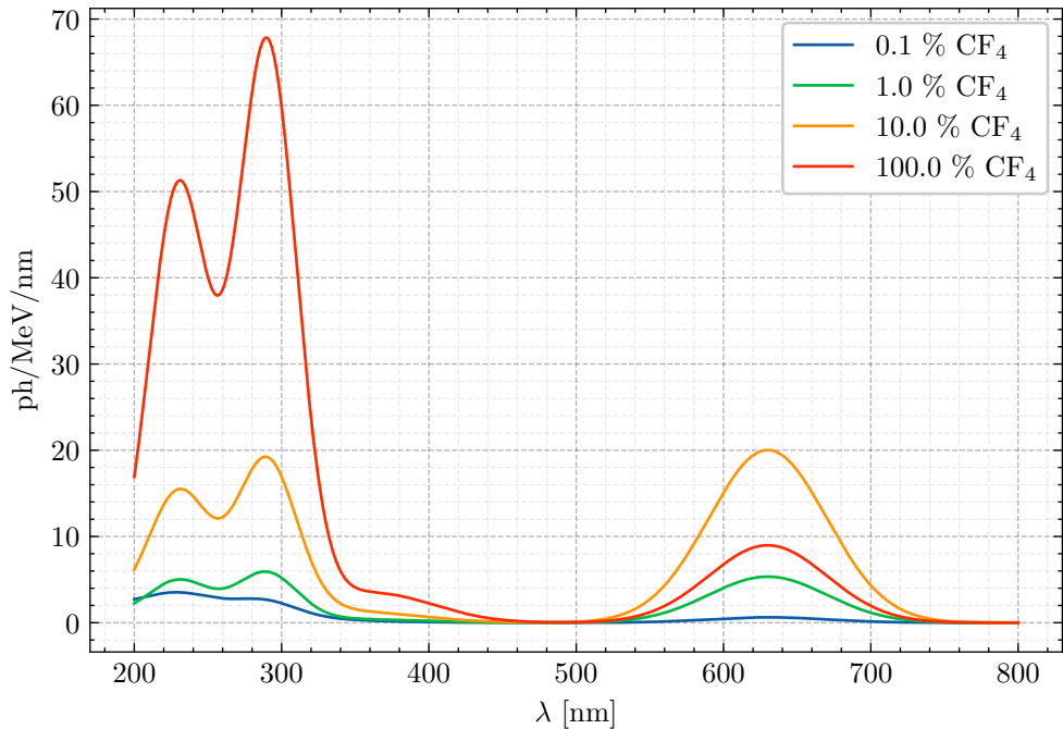
Primary Ar-CF 4 Spectra Prediction 3.0 bar
