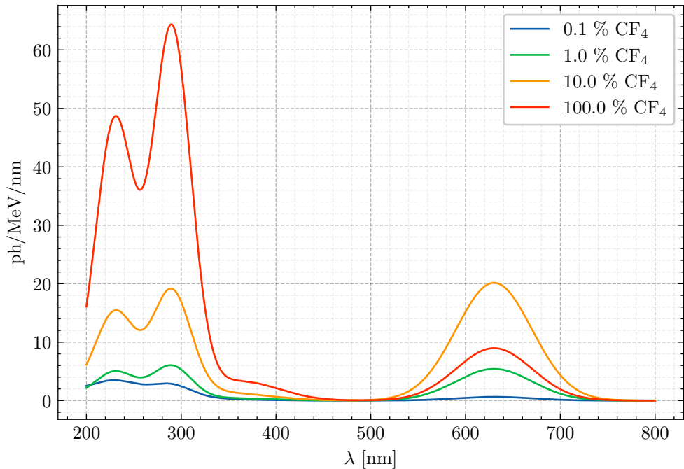
Primary Ar-CF 4 Spectra Prediction 4.0 bar
