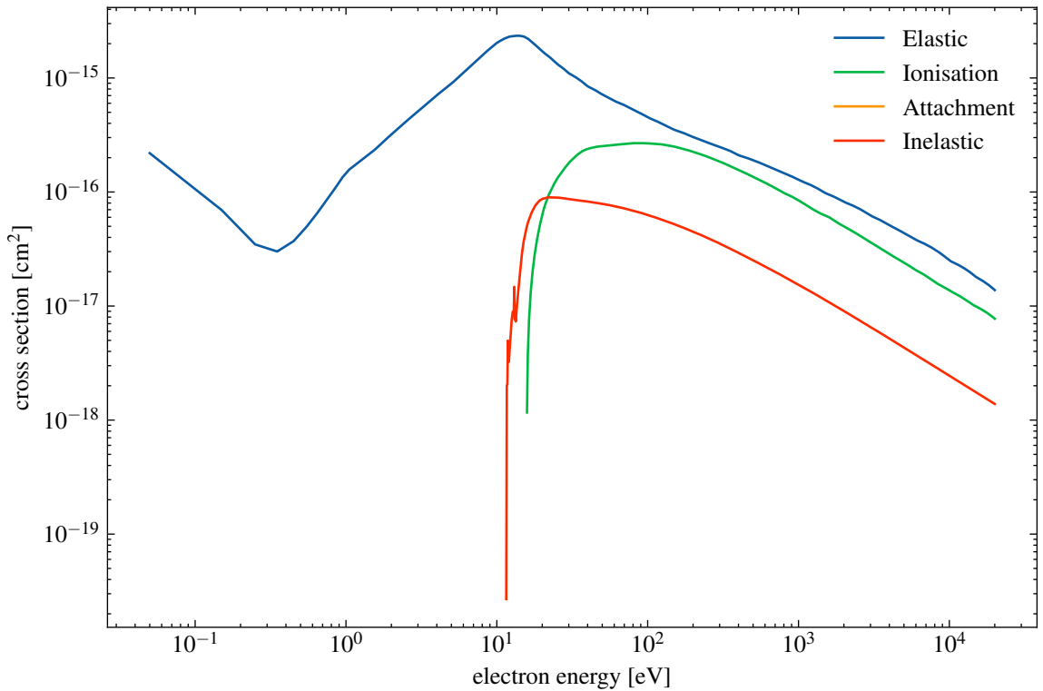
Argon Cross Section
