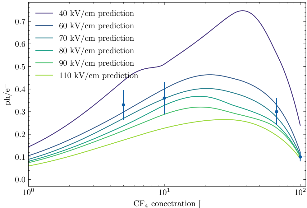
1 bar 100 gain secondary visible yield prediction for Ar/CF4 mixture
