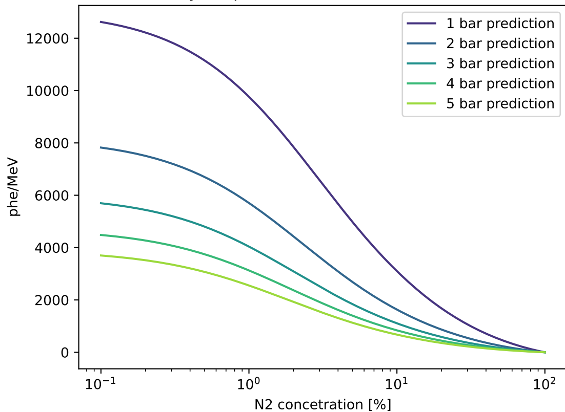
Ar-N 2 yield prediction IR (650 nm to 790 nm)
