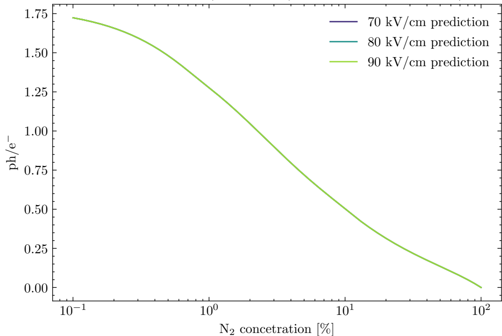
1 bar 10k gain secondary IR (680-785nm) Yield Prediction for Ar/N 2 mixture
