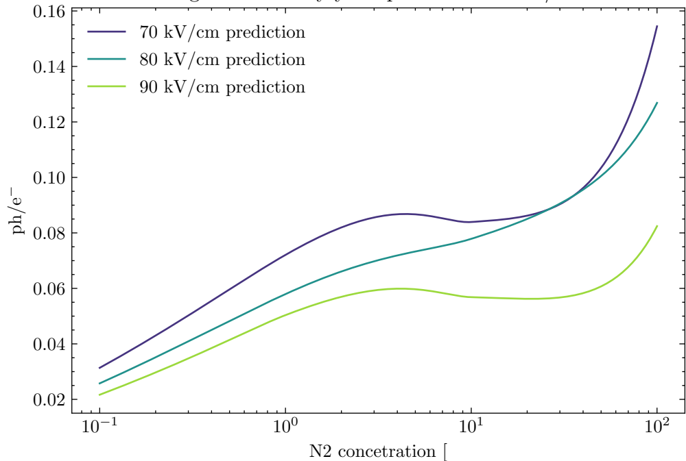
1 bar 10k gain secondary yield prediction for Ar/N2 mixture
