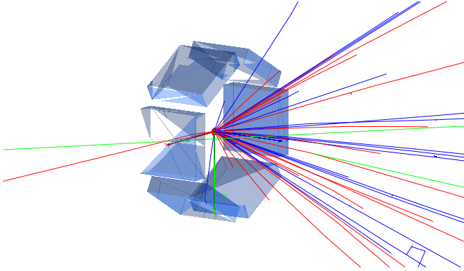
Fig. 2. Detector in the ATOMKI geometry, with 20 events of e^-e^+ production.
