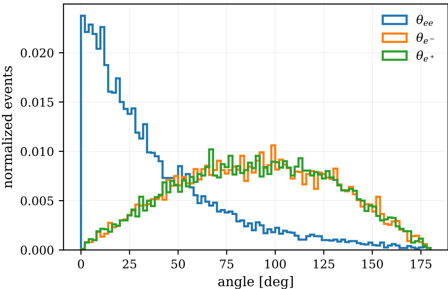
IPC-like background sampled angular variables
