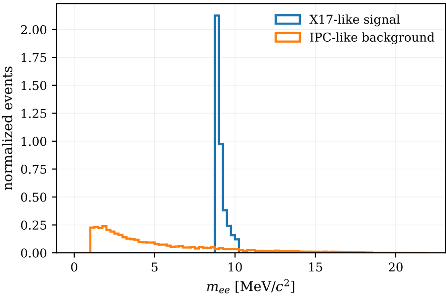
Generated invariant-mass templates
