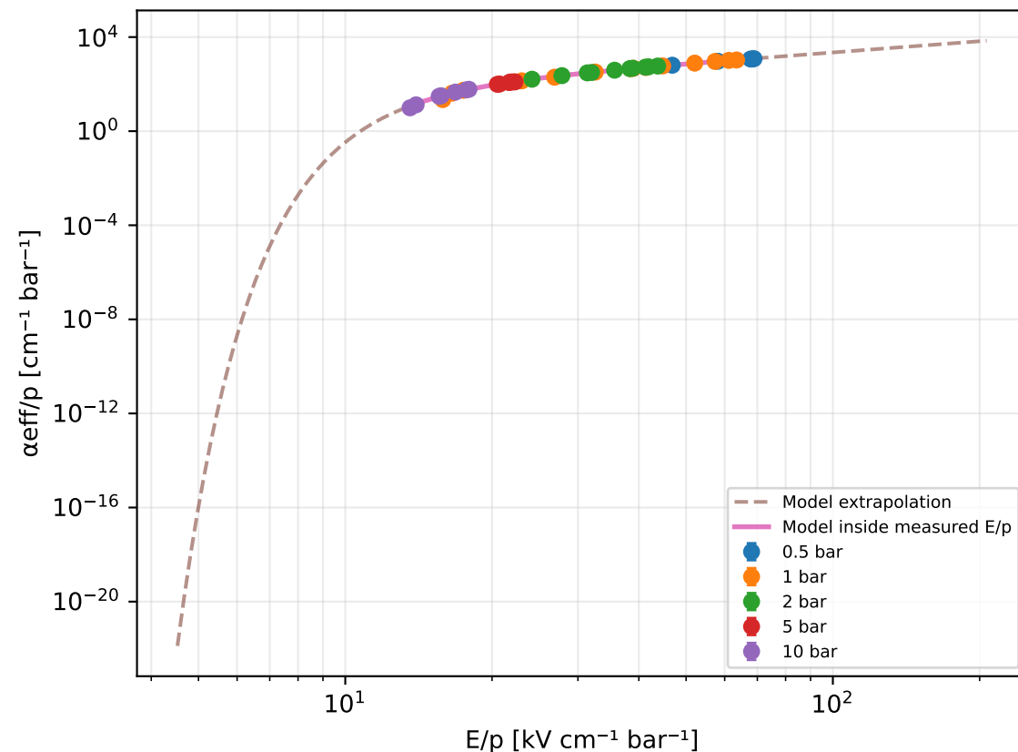
Reduced Townsend fit
