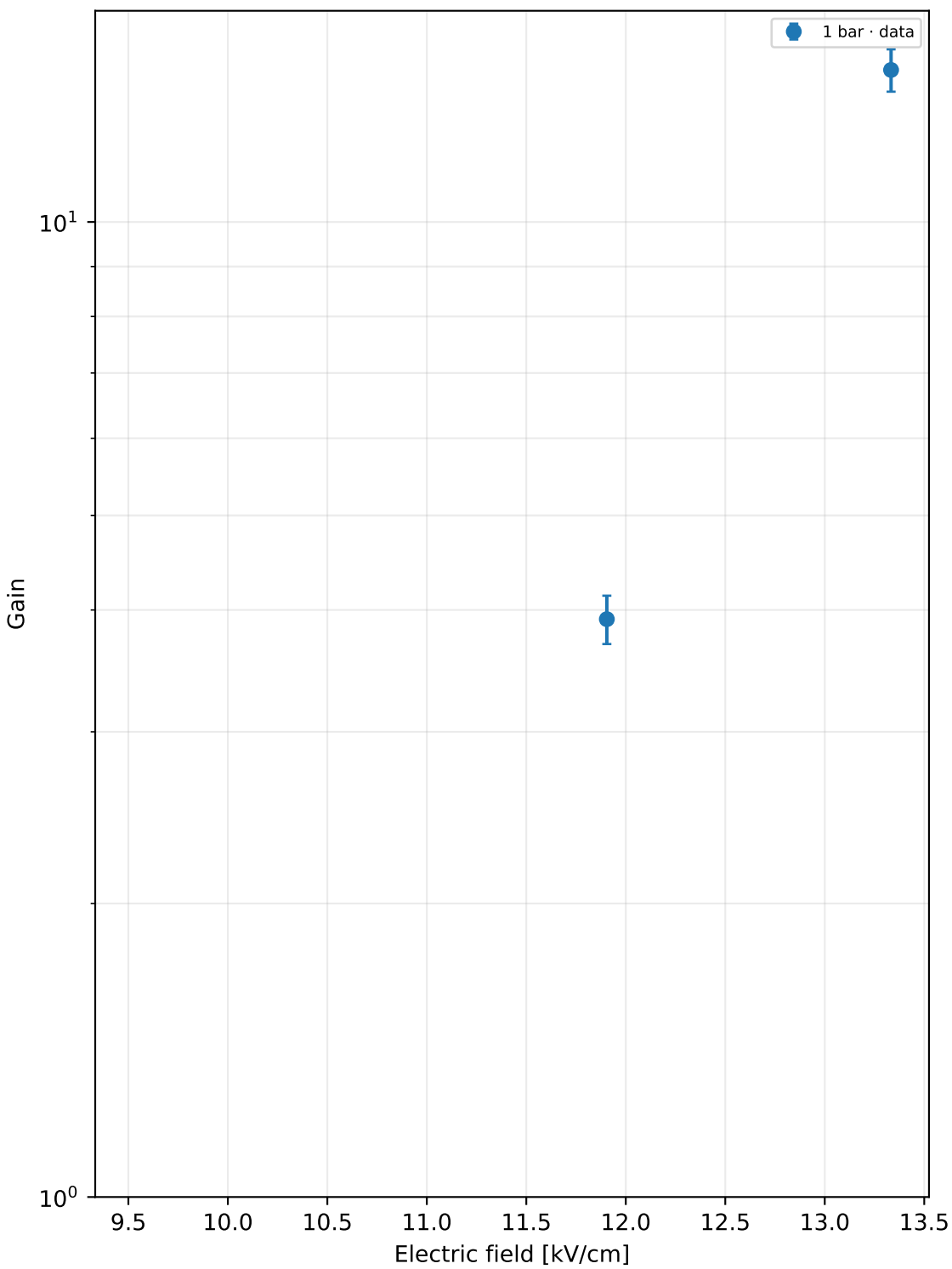
Gain vs electric field
