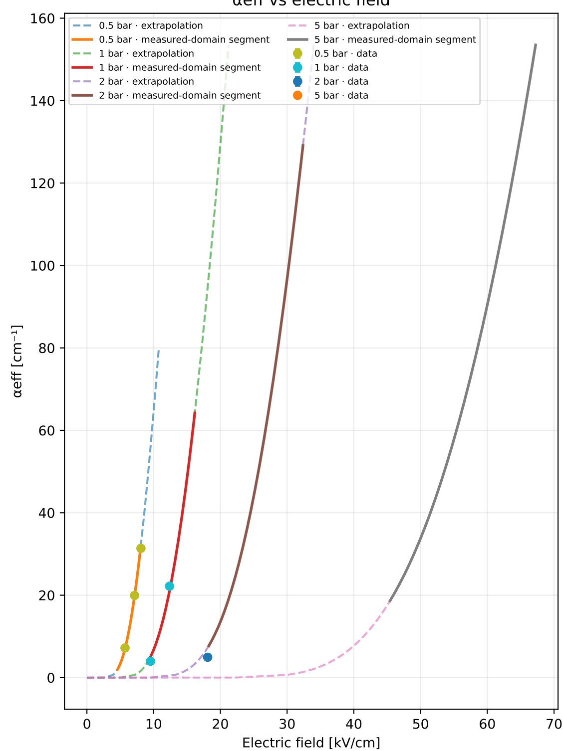
\alpha_{eff} vs electric field
