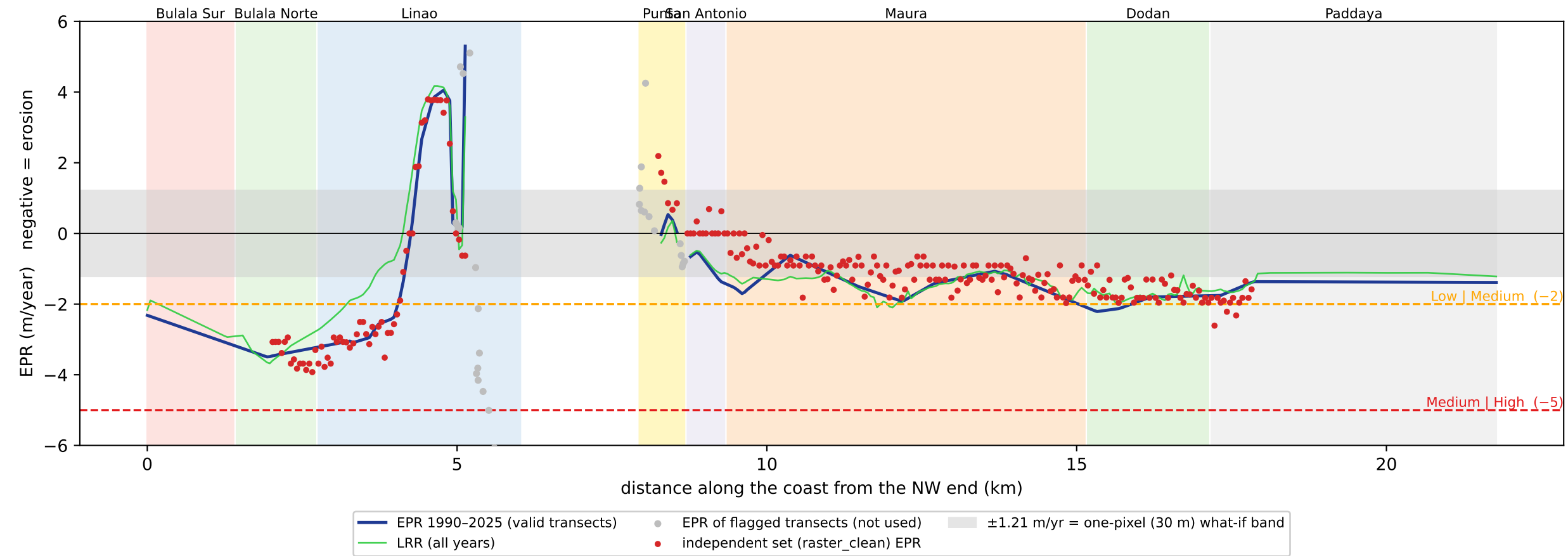
Shoreline change rate along the open coast of the eight study barangays, 1990-2025
