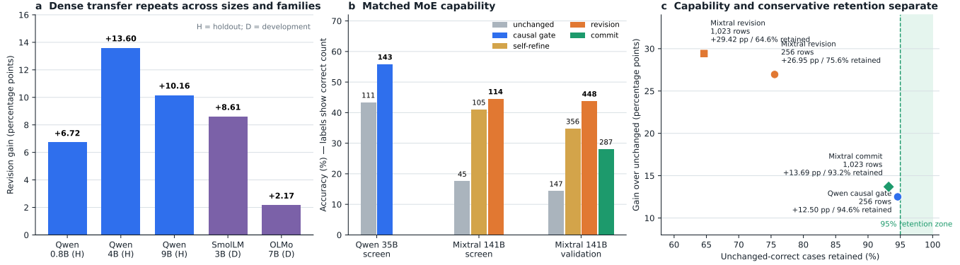
Figure 2: Capability transfer and its retention boundary. Dense gains repeat across sizes and families; both completed MoE families improve; and large aggregate gains can coexist with poor unchanged-case retention.
