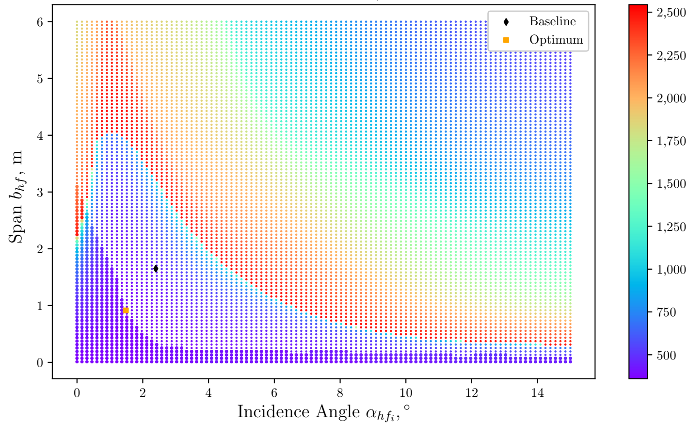
Takeoff Distance, m
