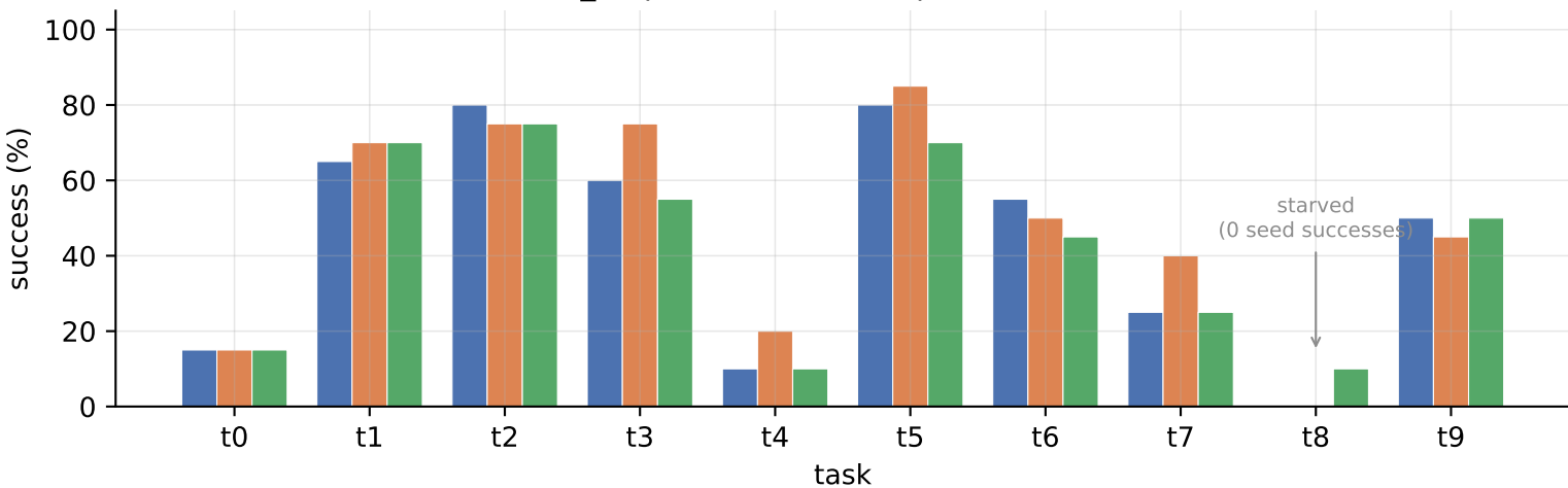
libero_10 per-task success (paired n=20/task)
