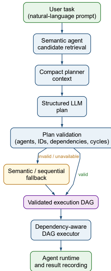
Figure 3.3: Planner, validation, and dependency-aware execution flow
