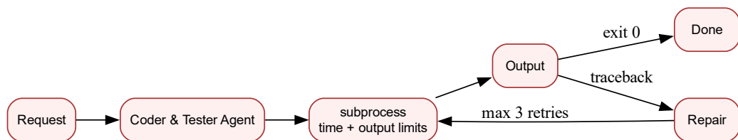
Figure 3.9: Sandboxed Python execution and bounded self-healing loop
