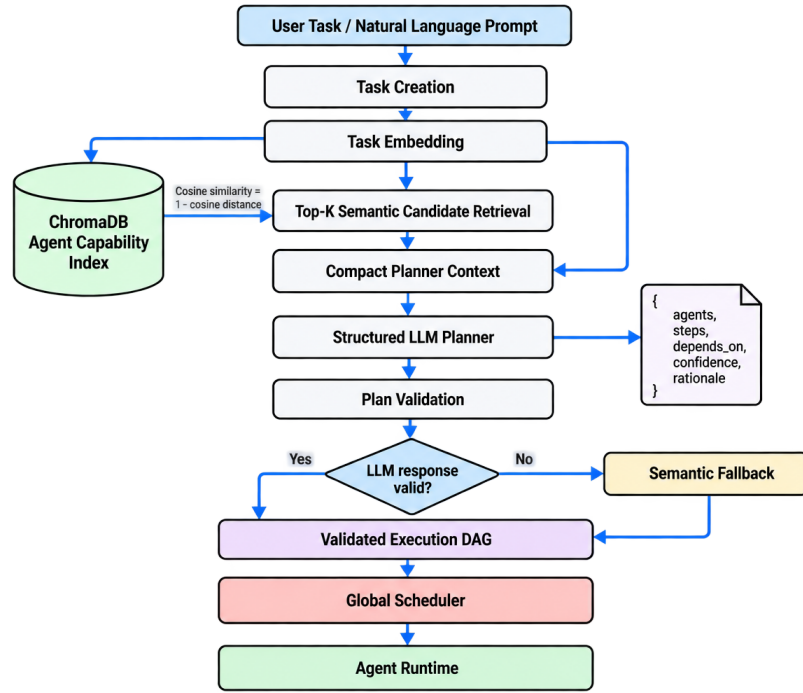
Figure 4.1: Optimized semantic planner and DAG construction
