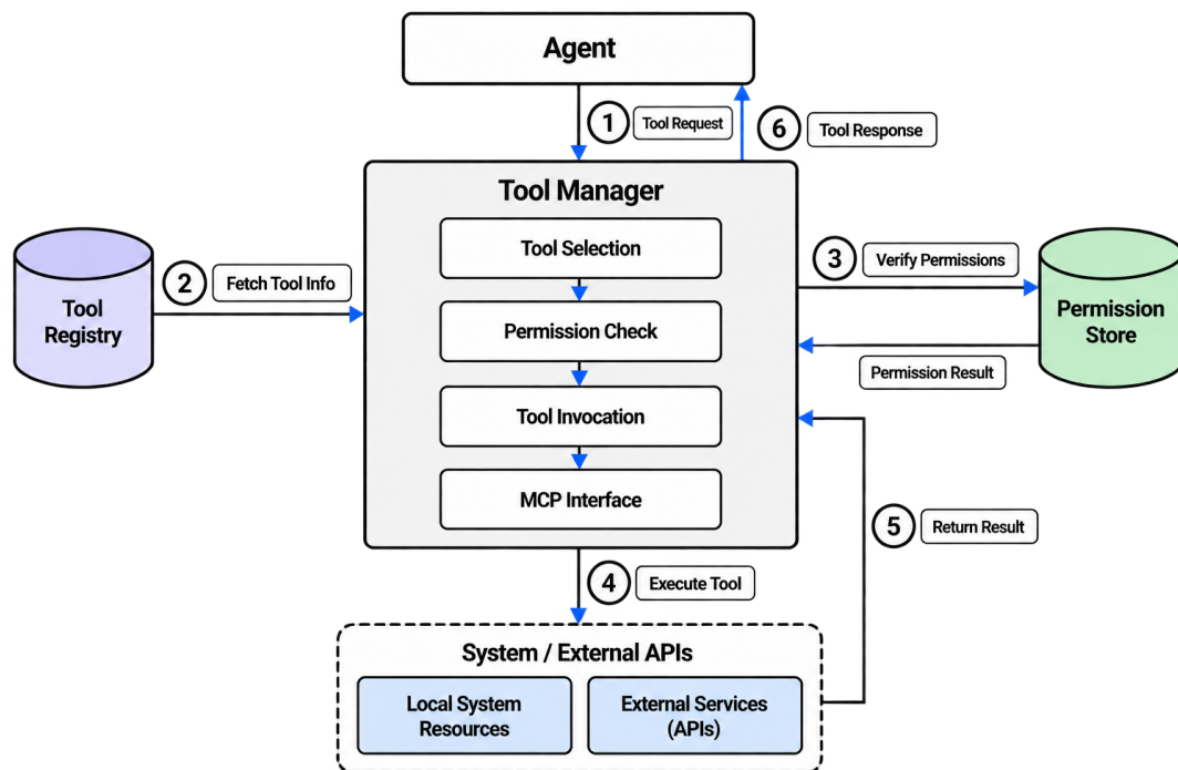
Figure 3.7: Tool selection, permission checking, invocation, and result return
