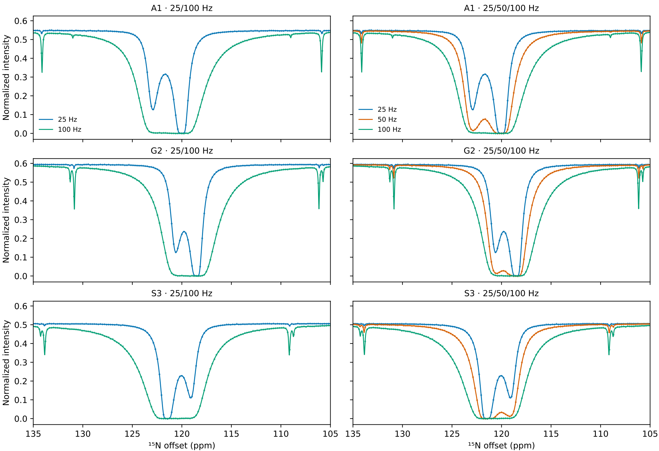
1.2 GHz full CEST profiles including 90^\circ\text{x}-240^\circ\text{y}-90^\circ\text{x} sidebands Dots: existing synthetic data; lines: refit with automatic peakwise proton relaxation
