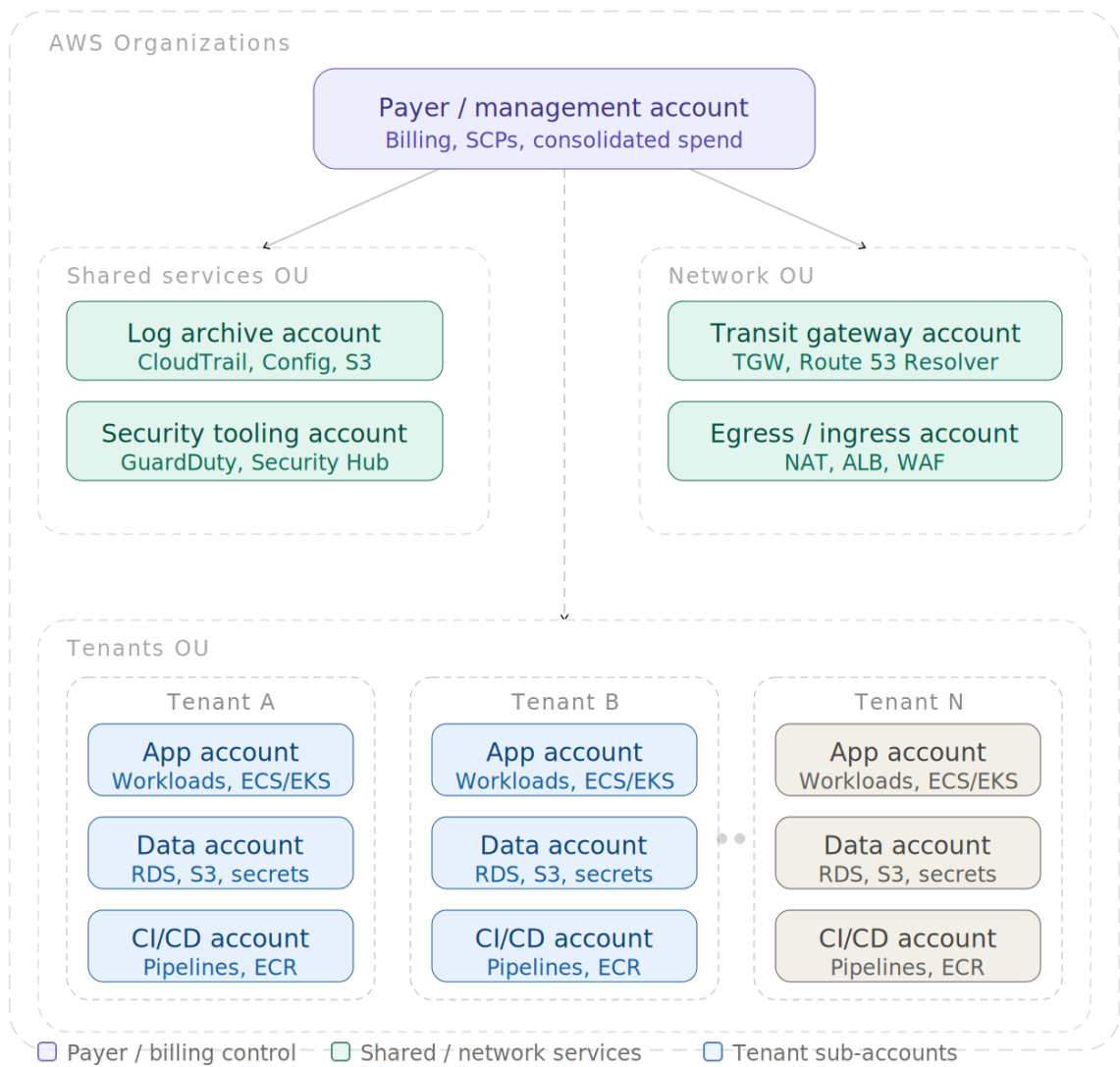
Figure 3: AWS Micro-Account Strategy — Organizations, Shared Services, and Per-Tenant Structure
