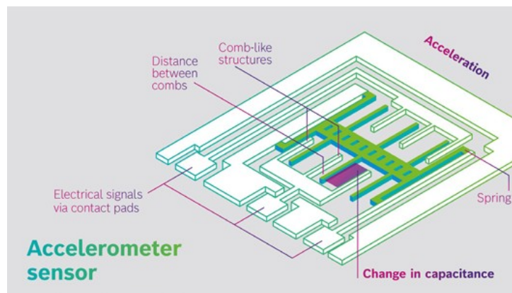
Fig. 4.2: MEMS Accelerometer Structure and Working Principle
