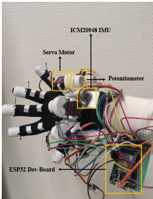
(a) IMU ICM20948 attached to the glove
