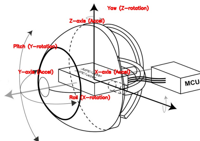
Fig. 4.1: IMU Axes Representation: Accelerometer (Linear Motion) and Gyroscope (Rotational Motion)
