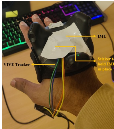
Fig. 7.1: Experimental setup showing the IMU attached to the Vive tracker to replicate the same positioning as on the glove
