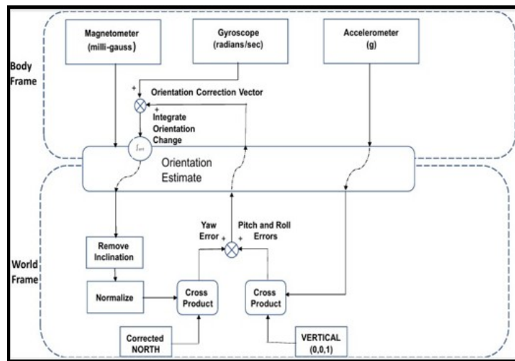
Fig. 5.2: Visual Overview of 9 DoF Quaternion-Based Complementary Filter
