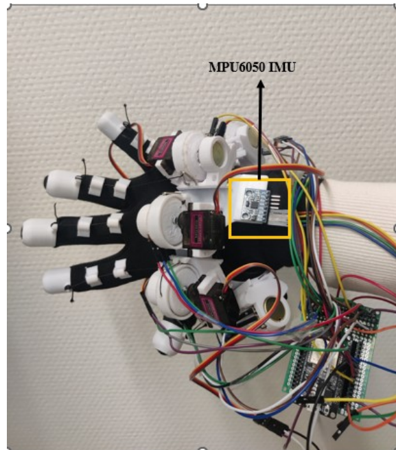
(b) IMU MPU6050 attached to the glove
