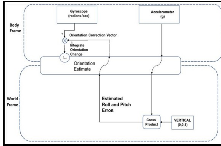
Fig. 5.1: Visual Overview of 6 DoF Quaternion-Based Complementary Filter
