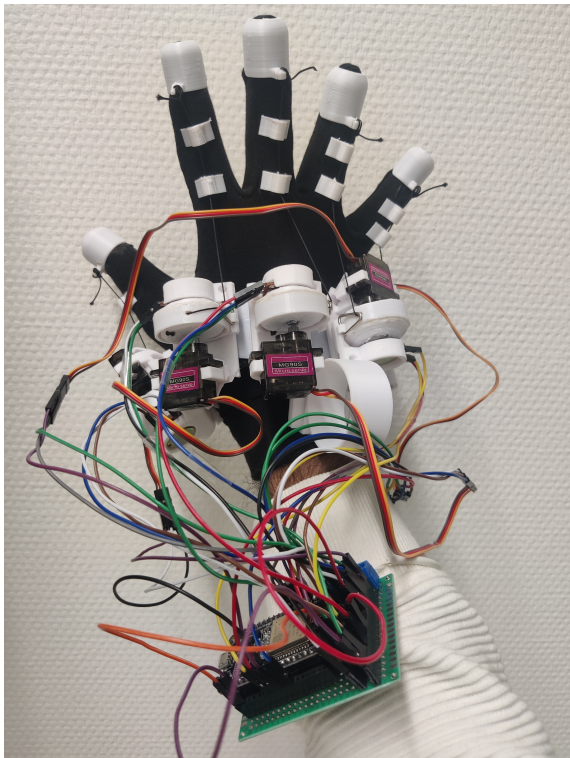
(a) Front view of the glove
