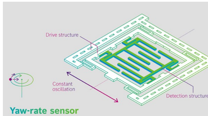
Fig. 4.3: MEMS Gyroscope Structure and Working Principle
