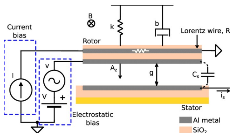
Fig. 4.4: MEMS Magnetometer Structure and Working Principle
