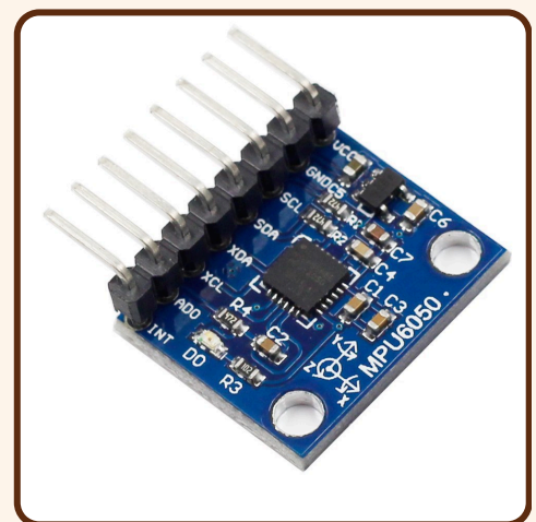
MPU6050 Price -: 164
