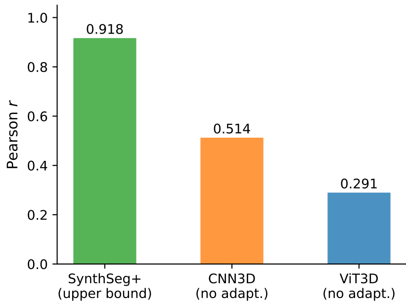
Pearson Correlation
