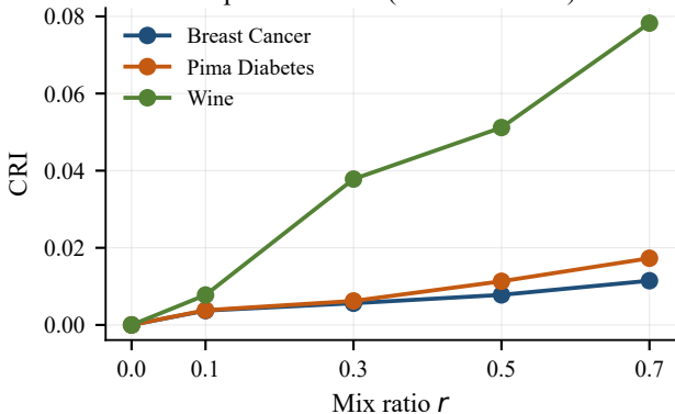
CRI vs. copula mix ratio (Random Forest)
