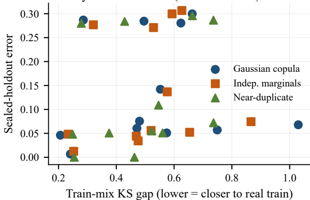
Fidelity vs. holdout risk (Pearson r=0.15 )
