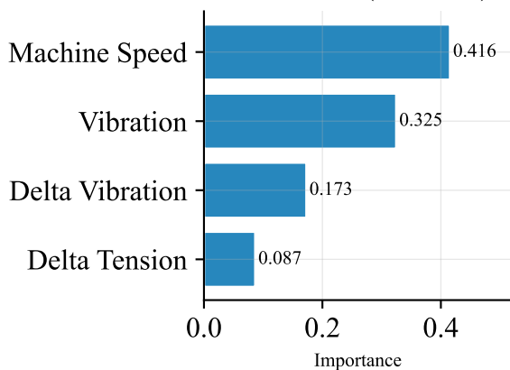
Fault Detector (Acc=98.2%)
