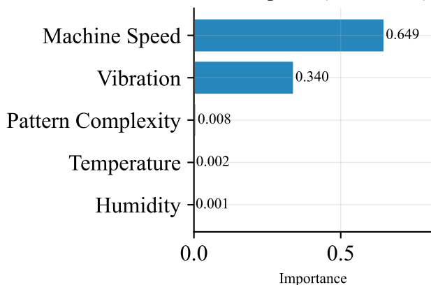
Defect Regressor (RMSE=0.005)
