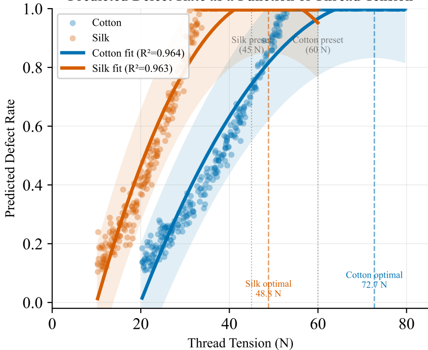
Predicted Defect Rate as a Function of Thread Tension
