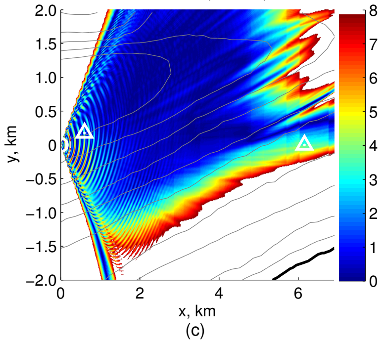
field difference ( z = 9 m), dB
