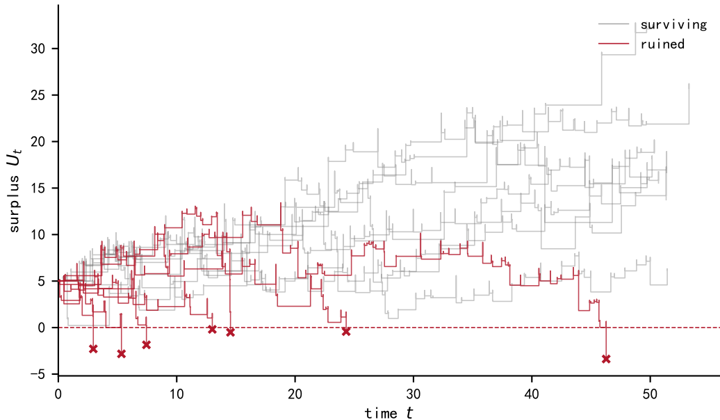
Cramer-Lundberg surplus ( \theta=0.2 , ruined: 7/15)
