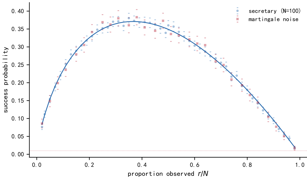
Secretary problem vs martingale control
