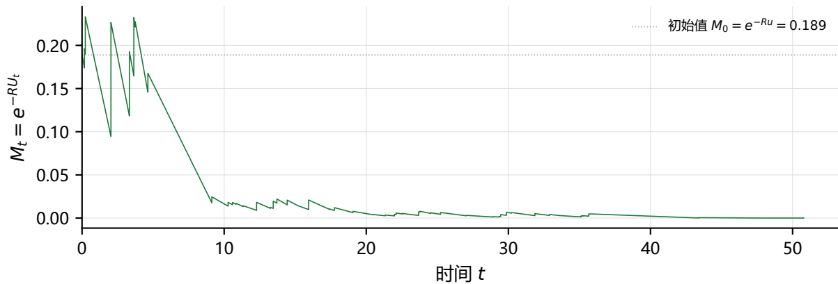
指数鞅 ( R = 0.3333 )
