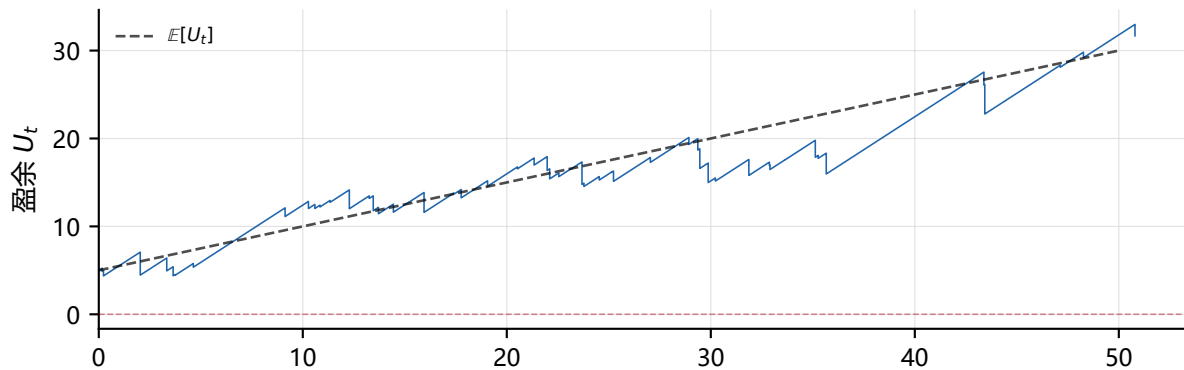
指数鞅 ( R = 0.3333 )
