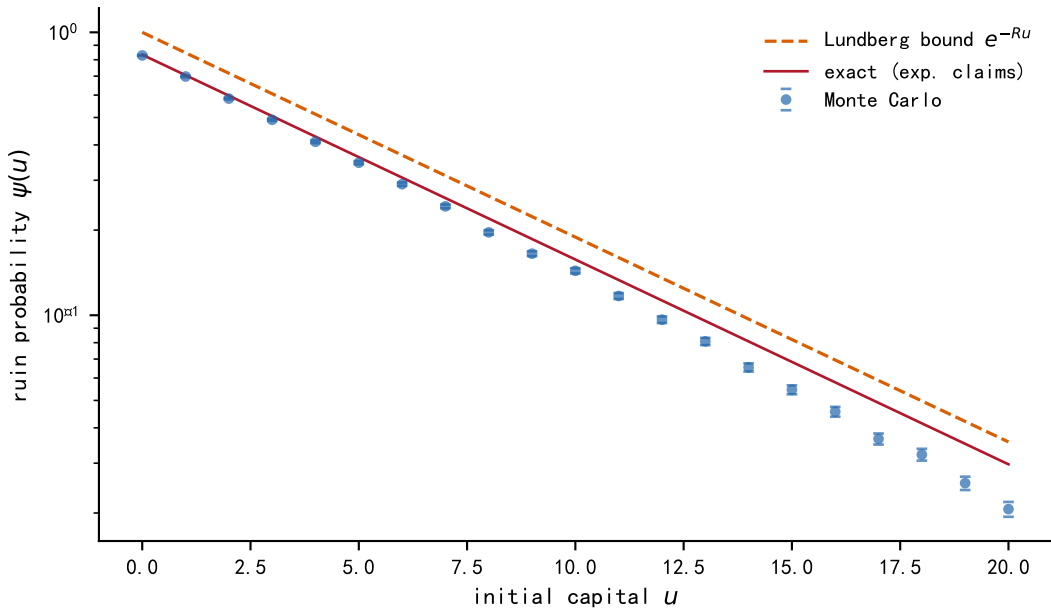
Ruin probability vs initial capital (semi-log)
