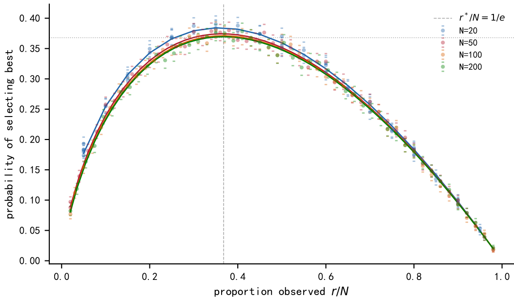
Secretary problem: success rate vs r/N
