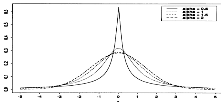
Figure 2.2.5 Densities of s\alpha s rvs with c = 1 .
