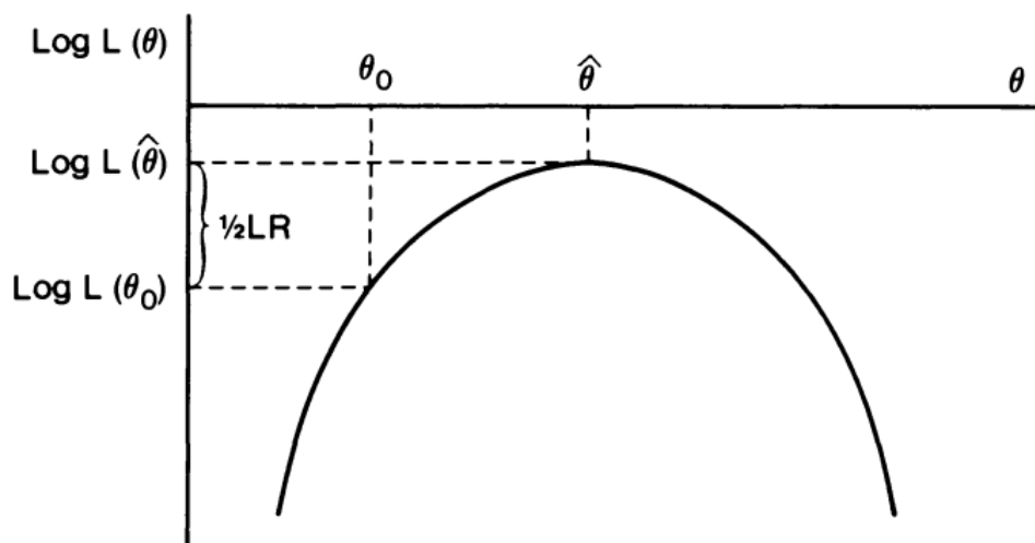
Figure 1. The Likelihood Ratio Test
