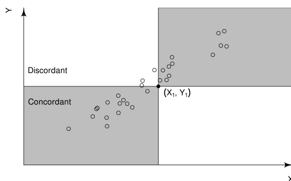
图 10.1: Kendall's \tau 中一致与不一致的样本对。图片来自 https://en.wikipedia.org/wiki/Kendall_rank_correlation_coefficient
