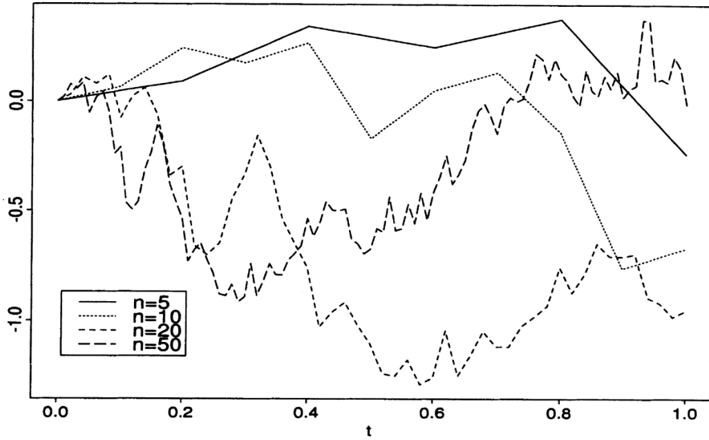
Figure 2.4.3 Visualisation of the Donsker invariance principle: sample paths of the process S_n(\cdot) for the same realisation of (X_n) for n = 5, 10, 20, 50 .
