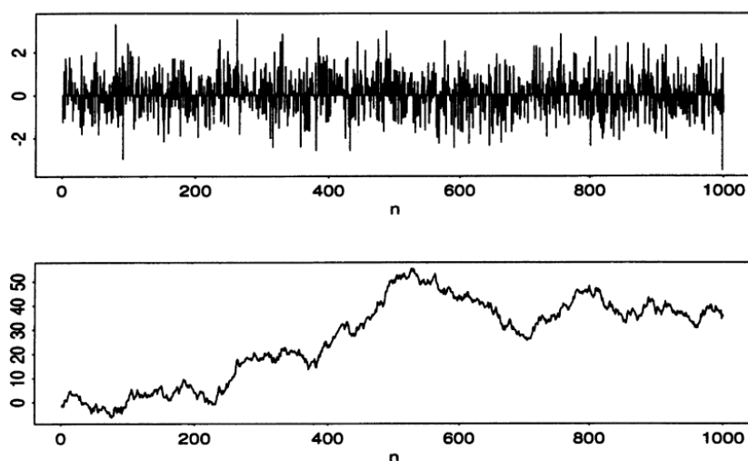
Figure 2.2.11 One sample path of the process (X_n) (top) and of the corresponding path (S_n) (bottom) for X with a standard normal distribution.
