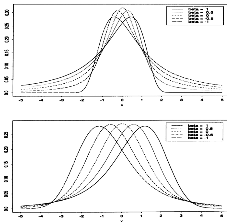
Figure 2.2.6 Densities of 1- and of 1.5-stable rvs (top, bottom) with c = 1 .
