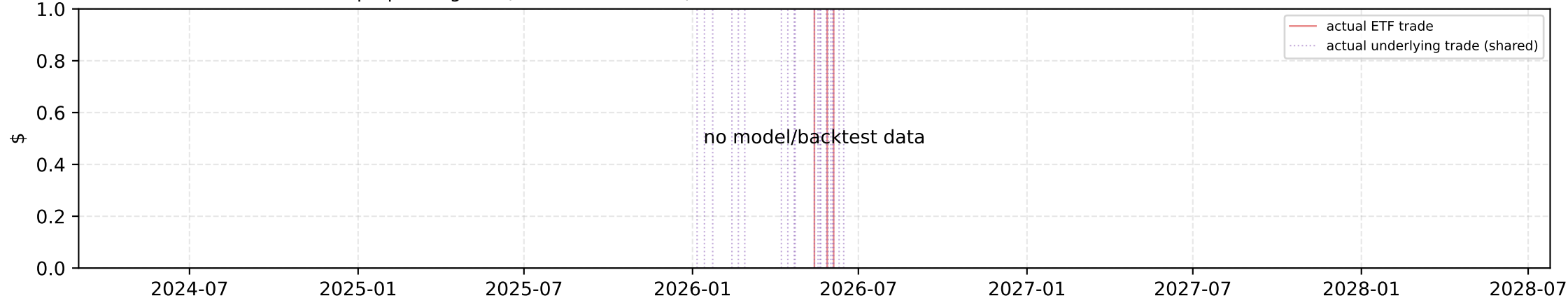
Hedge ratio over time
