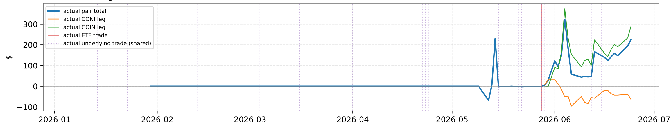
Model/backtest PnL scaled to proposed gross (model unavailable)
